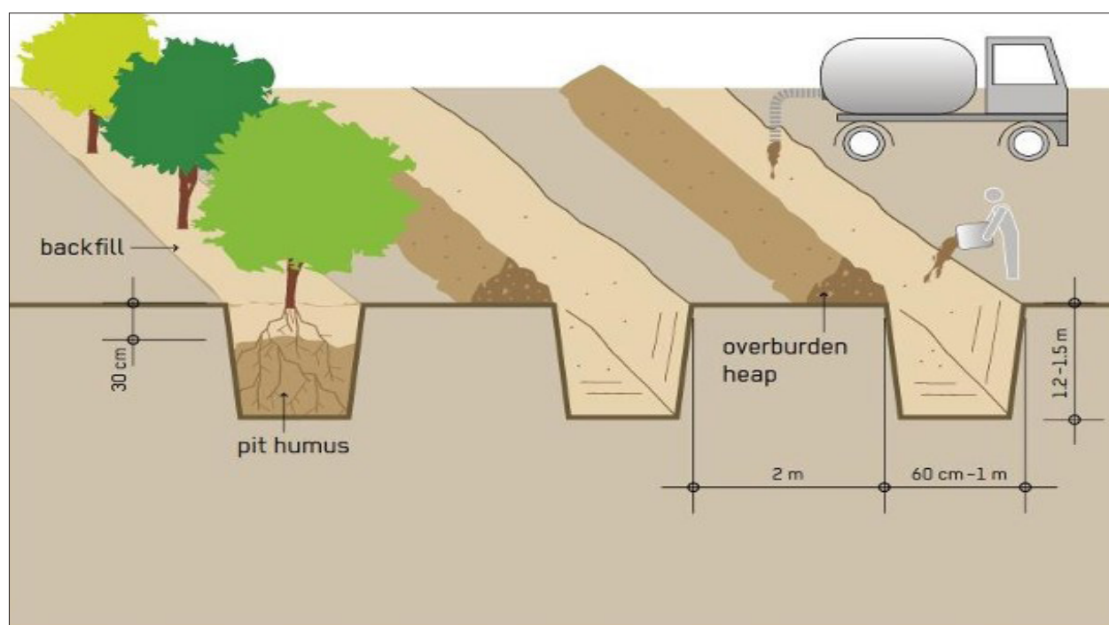
Figure 1: Design of DRE trenches
